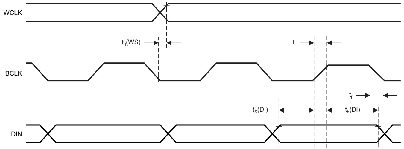
Figure 1. I 2 S/LJF/RJF Timing in Master Mode
