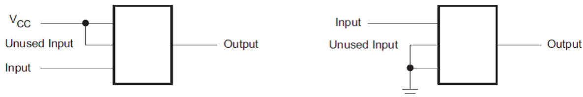
Figure 9-3. Layout Example
