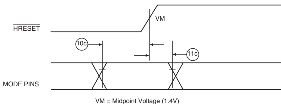
Figure 11-3. Mode Select Input Timing Diagram
