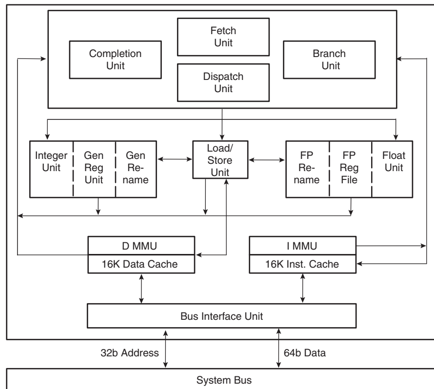
Figure 3-1. Block Diagram
