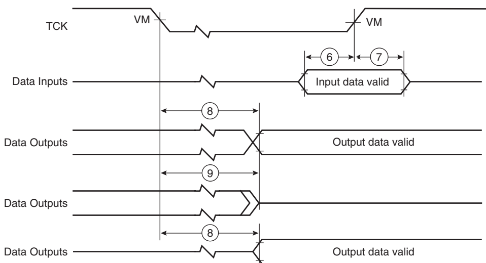
Figure 11-7. Boundary-scan Timing Diagram
