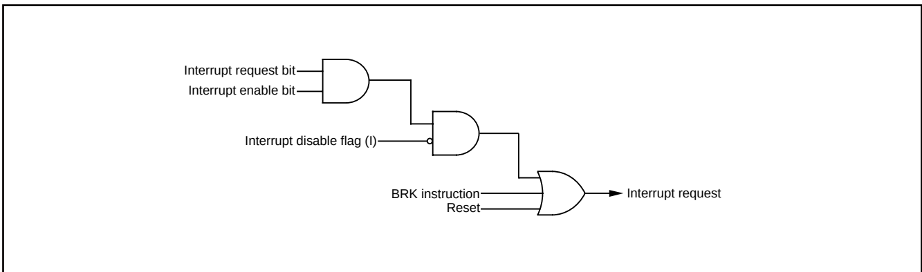
Fig. 18 Interrupt control
