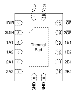
Figure 5-2. BQB Package 16-Pin WQFN Transparent Top View
