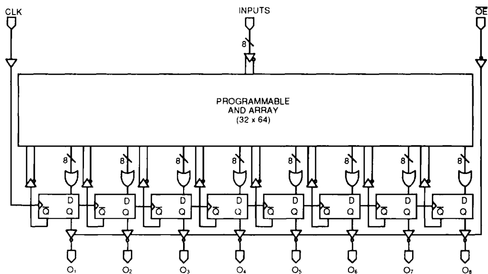
PAL16R8
