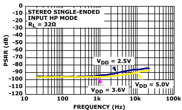
FIGURE 23. POWER SUPPLY REJECTION RATIO (HEADPHONES) vs FREQUENCY
