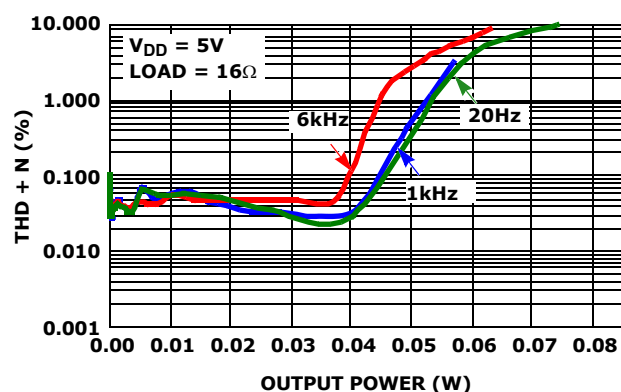
FIGURE 4. TOTAL HARMONIC DISTORTION PLUS NOISE vs POWER (HEADPHONE)
