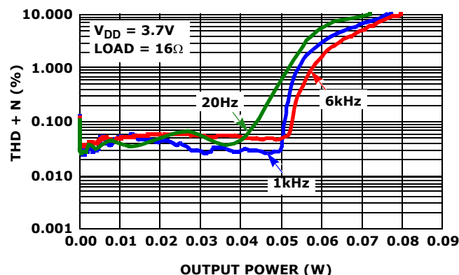
FIGURE 6. TOTAL HARMONIC DISTORTION PLUS NOISE vs POWER (HEADPHONE)
