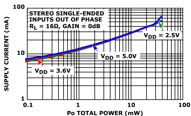
FIGURE 14. SUPPLY CURRENT (HEADPHONES) vs TOTAL OUTPUT POWER
