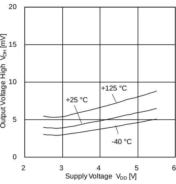
Figure 3. Output Voltage High vs Supply Voltage (R L =10 kΩ)
