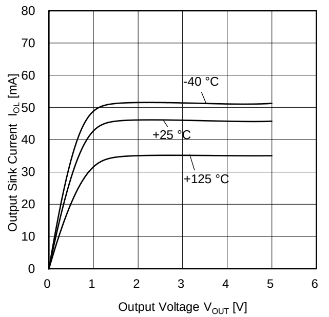
Figure 8. Output Sink Current vs Output Voltage ( V_{DD}=5\text{ V} )
