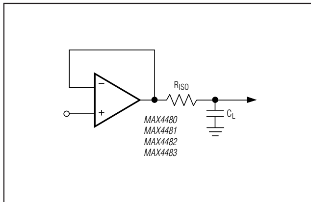
Figure 3. Capacitive-Load-Driving Circuit
