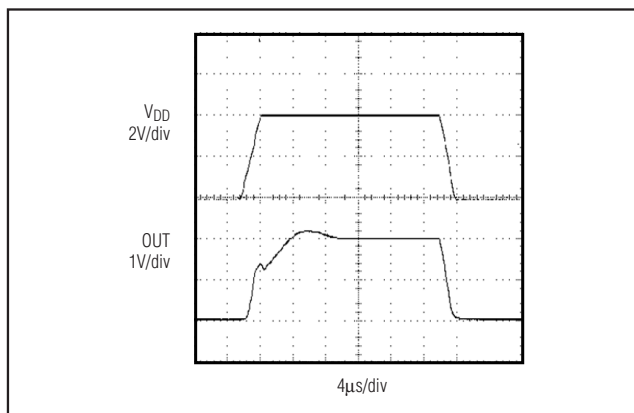
Figure 5. Power-Up/Down Waveform
