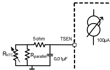
Figure 42: Temperature Sense NTC Network
