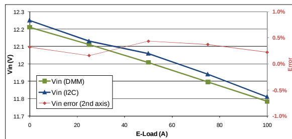
Figure 46: I2C Input Voltage Measurements
