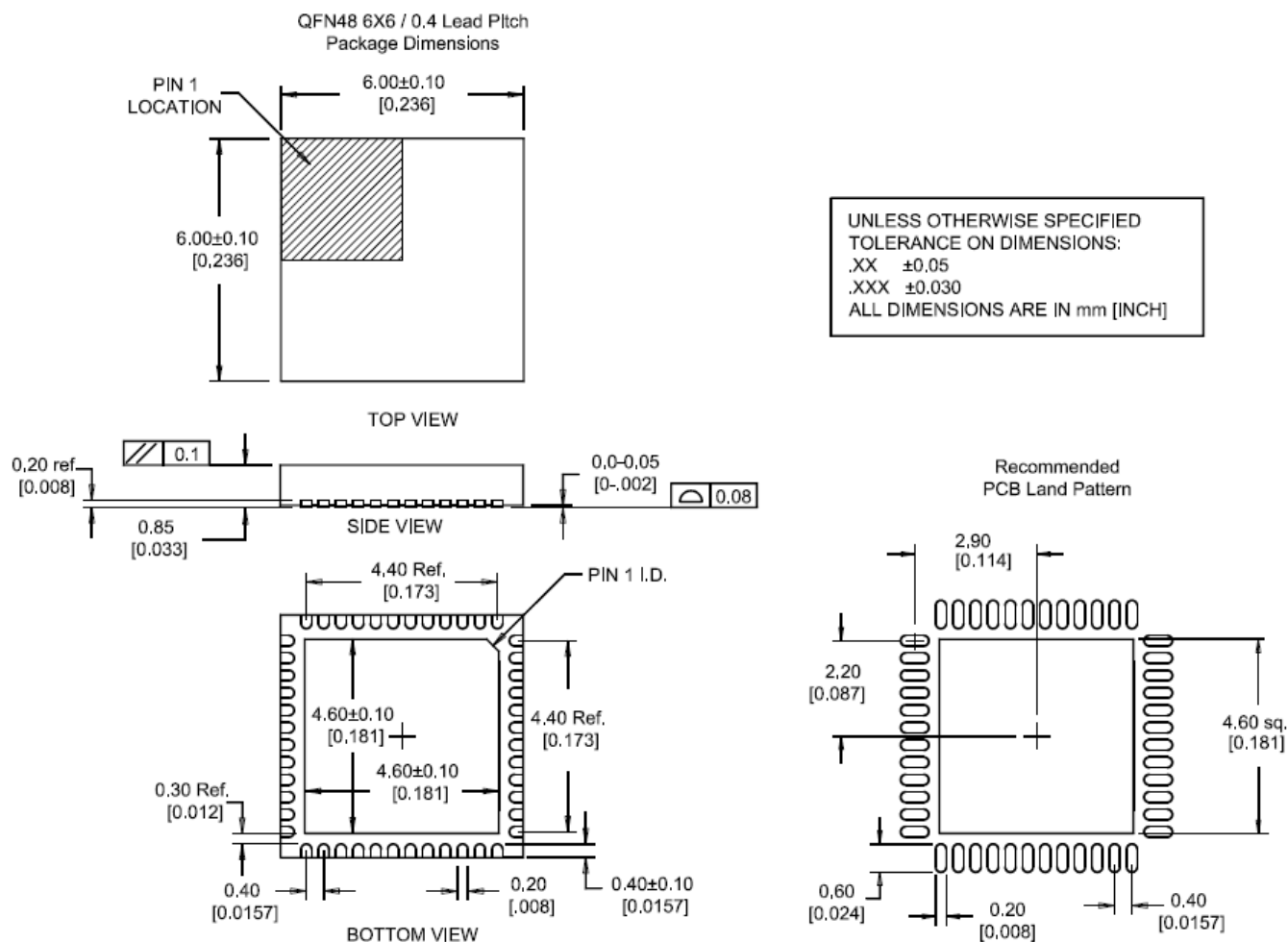
Figure 67: Package Dimensions
