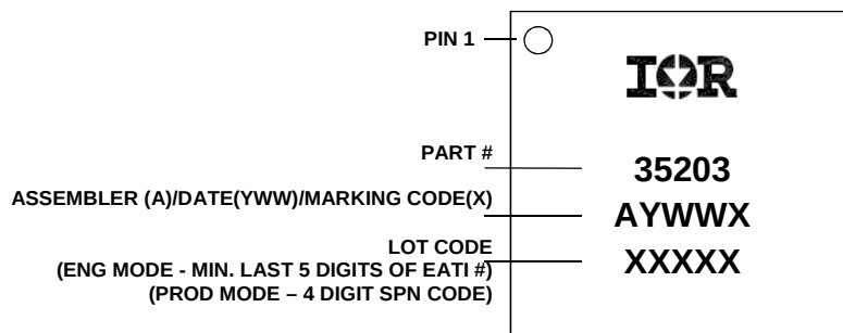
Figure 66: Package Marking
