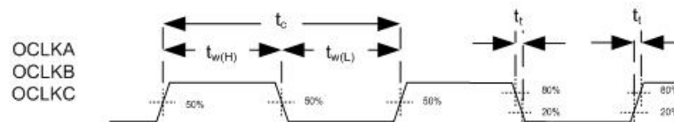
Figure 5. Programmable Output Clocks
