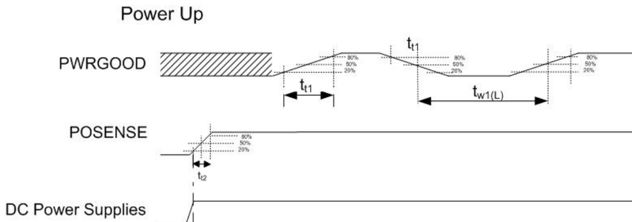
Figure 2. Power Up
