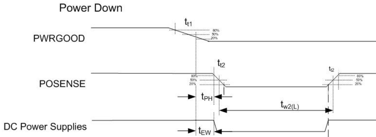
Figure 3. Power Down
