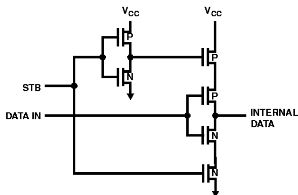
FIGURE 1. 82C82/83H
