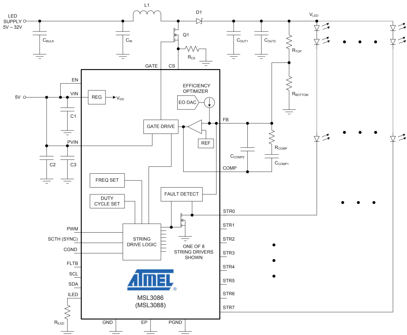
Figure 1. MSL 3086/MSL 3088 Block Diagram
