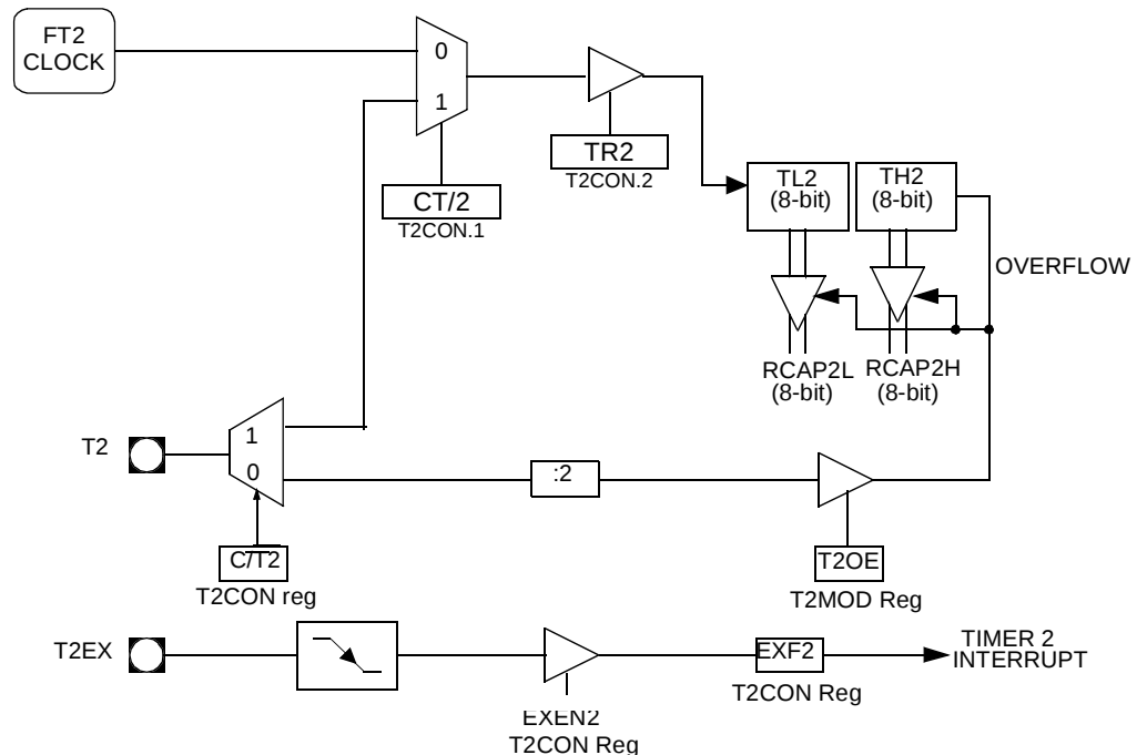
Figure 30. Clock-Out Mode
