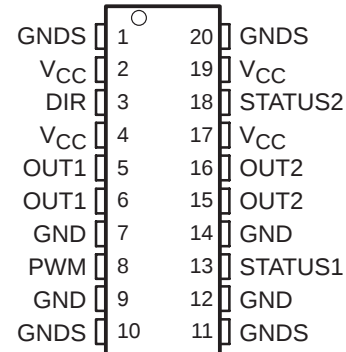
DWP PACKAGE (TOP VIEW)
