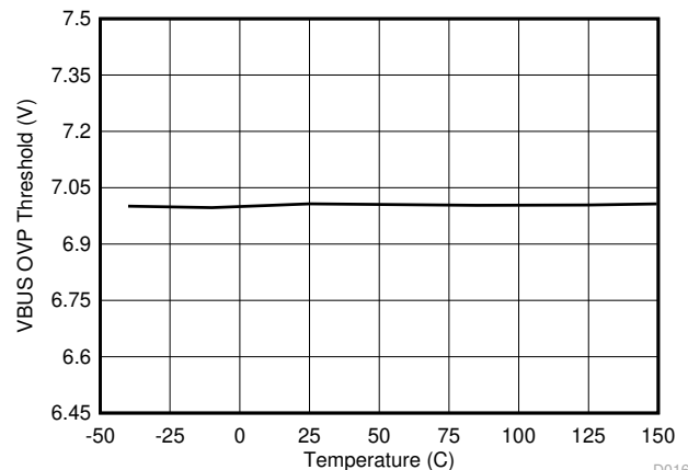
Figure 8-18. VBUS Overvoltage Protection Threshold vs Junction Temperature
