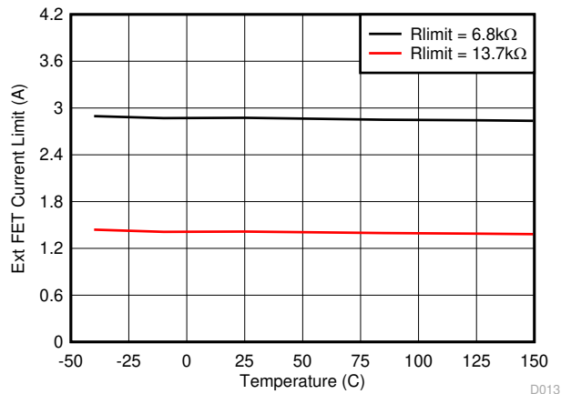
R_{SNS} = 15\text{ m}\Omega R_{SET} = 300\text{ }\Omega Figure 8-13. External FET Current Limit vs Junction Temperature
