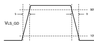
Figure 9-2. NFET Gate Drive Rise and Fall Time
