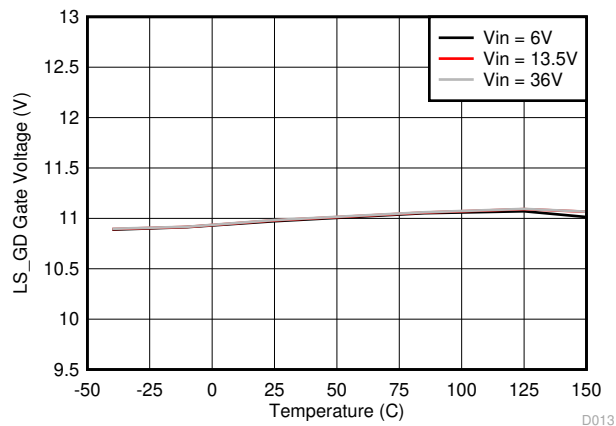
V_{CSN/OUT} = 5.1\text{ V} R_{IMON} = 0\text{ k}\Omega Figure 8-15. LS_GD Gate Voltage vs Junction Temperature
