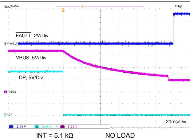
Figure 11-31. DP Short to BAT Recovery
