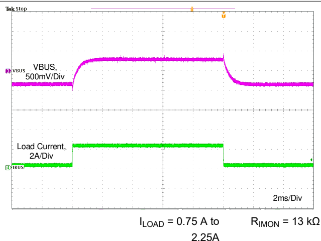
Figure 11-11. Load Transient With Cable Compensation
