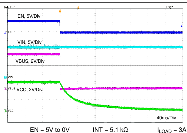
Figure 11-19. Shutdown Relate to EN
