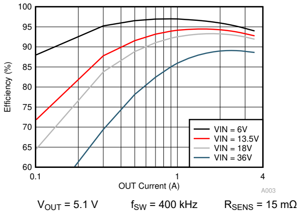
Figure 11-4. Efficiency With Sense Resistor
