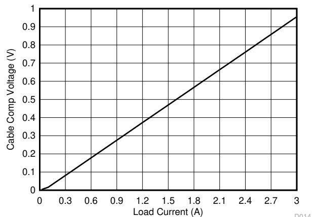
R_{SNS} = 15\text{ m}\Omega R_{SET} = 300\text{ }\Omega R_{IMON} = 13\text{ k}\Omega Figure 8-17. Cable Compensation Voltage vs Load Current
