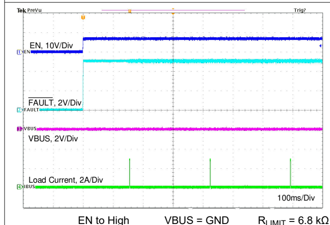
Figure 11-24. Enable Into Short With External FET
