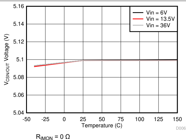
Figure 8-6. V_{CSN/OUT} Voltage vs Junction Temperature
