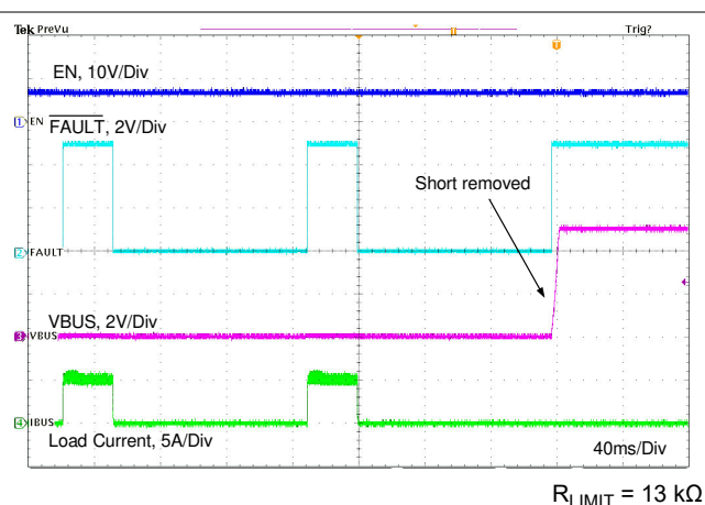
Figure 11-21. Short Circuit Recovery Without External FET
