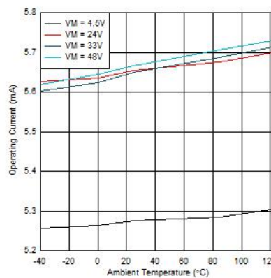
Figure 6-5. Operating Current over Temperature
