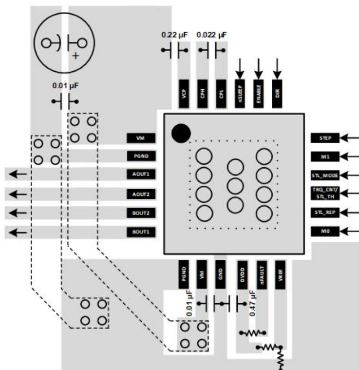
Figure 10-2. QFN Layout Example
