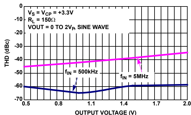
FIGURE 26. THD (dBc) vs OUTPUT VOLTAGE ( V_{p,p} )
