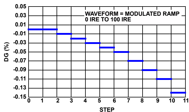
FIGURE 11. DIFFERENTIAL GAIN
