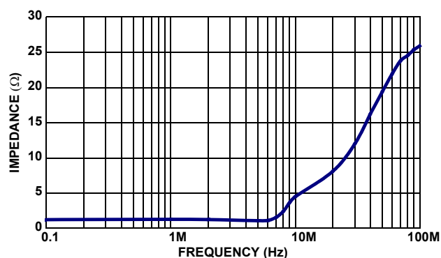
FIGURE 9. OUTPUT IMPEDANCE vs FREQUENCY
