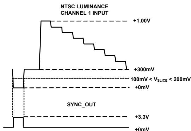
FIGURE 28. SYNC DETECTOR SLICE LEVEL
