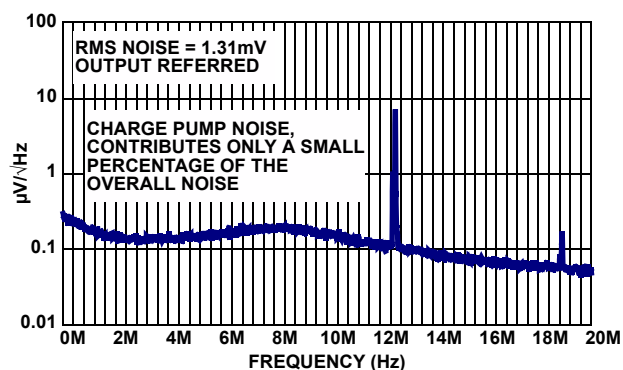
FIGURE 24. NOISE SPECTRUM
