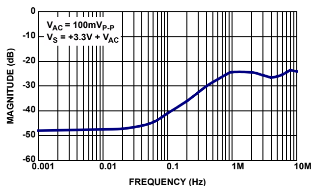
FIGURE 10. POWER SUPPLY REJECTION RATIO vs FREQUENCY
