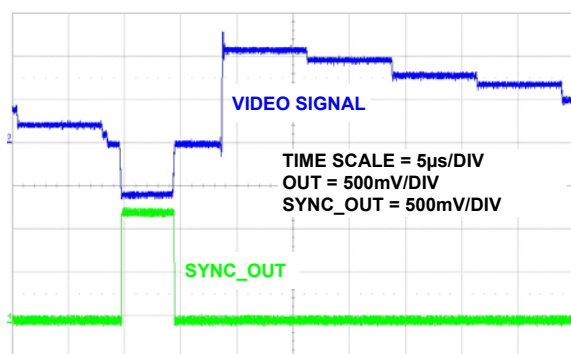
FIGURE 19. SYNC_OUT SIGNAL
