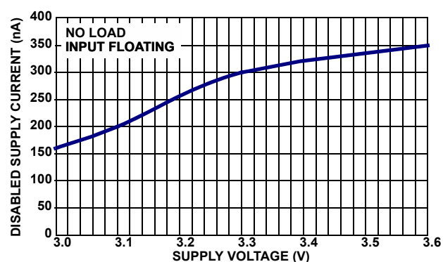
FIGURE 8. DISABLED SUPPLY CURRENT vs SUPPLY VOLTAGE
