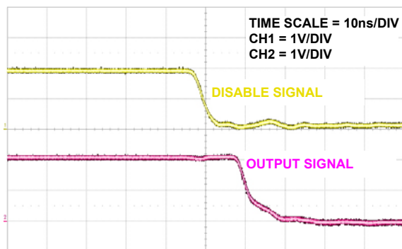
FIGURE 13. DISABLE TIME
