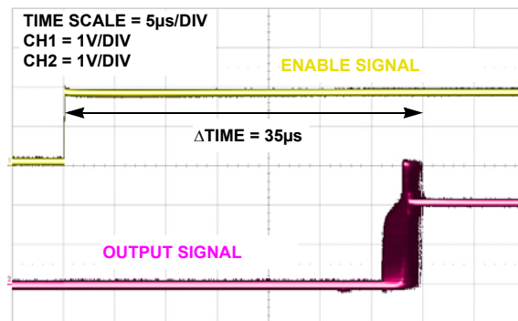
FIGURE 14. ENABLE TIME
