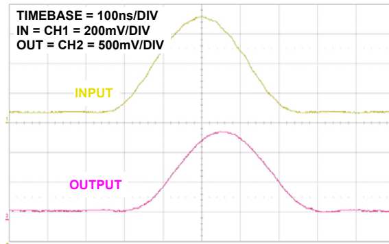
FIGURE 16. 2T RESPONSE
