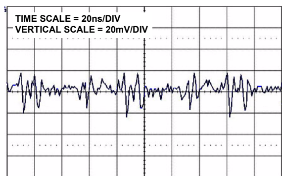
FIGURE 25. CHARGE PUMP FEEDTHROUGH AT AMPLIFIER OUTPUT
