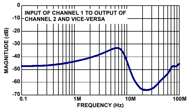
FIGURE 6. LUMA-TO-CHROMA CROSSTALK
