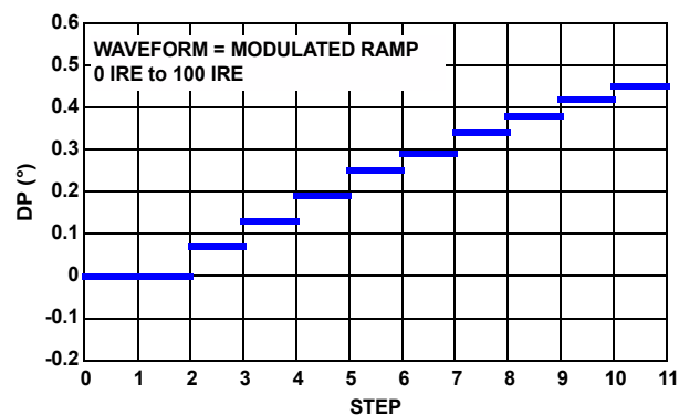
FIGURE 12. DIFFERENTIAL PHASE
