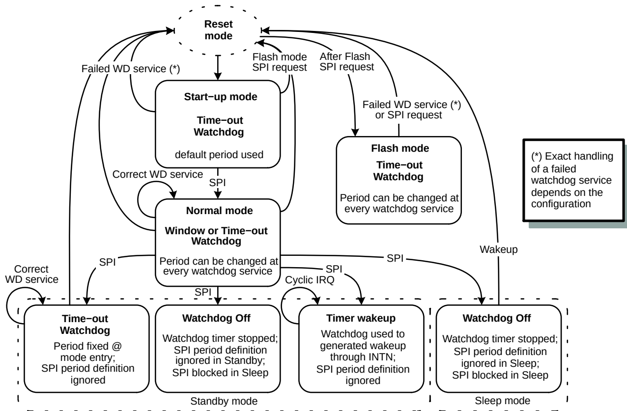
Figure 14. Watchdog Modes
