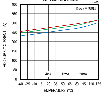
VCC SUPPLY CURRENT (SYSTEM LEVEL) vs. TEMPERATURE
