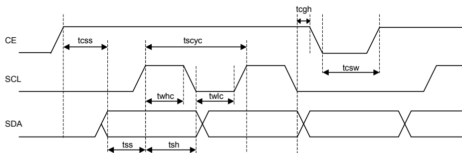
Figure 4. Timing diagram (SPI format)
