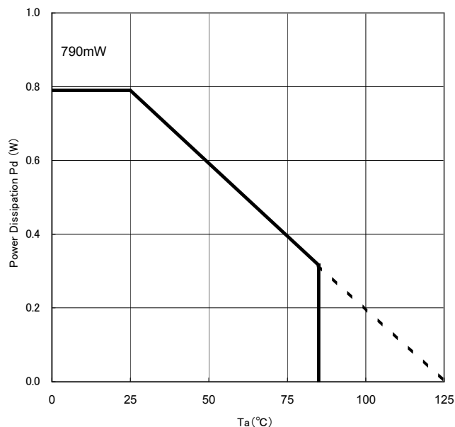
Figure 22. Power dissipation
