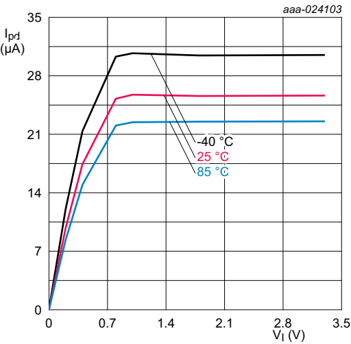
Fig 29. Typical pull-down current I_{PD} versus input voltage V_i
