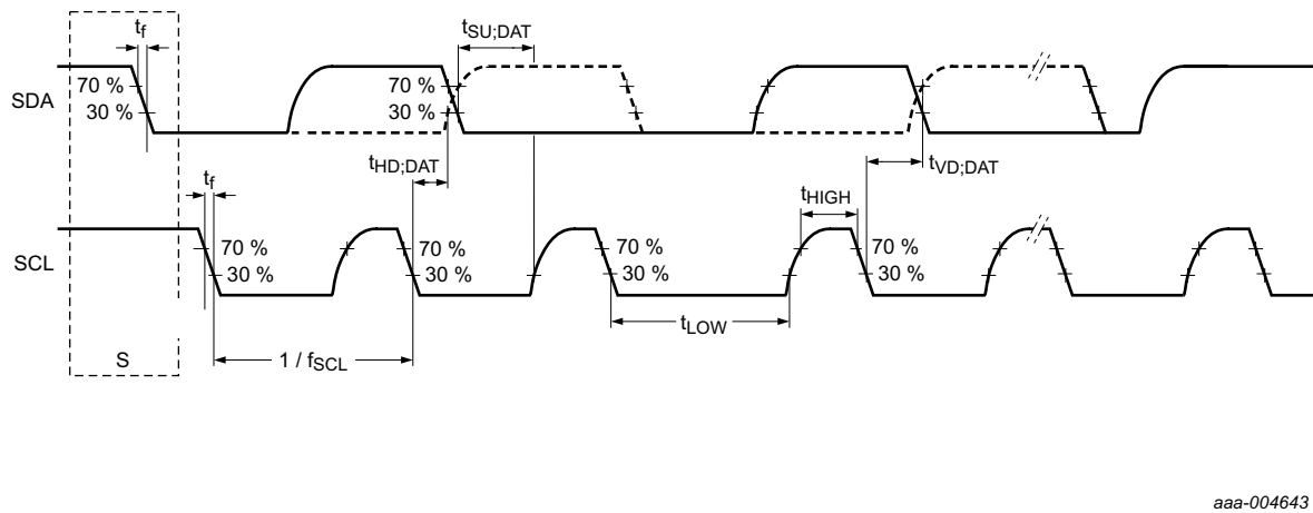
Fig 33. I 2 C-bus pins clock timing
