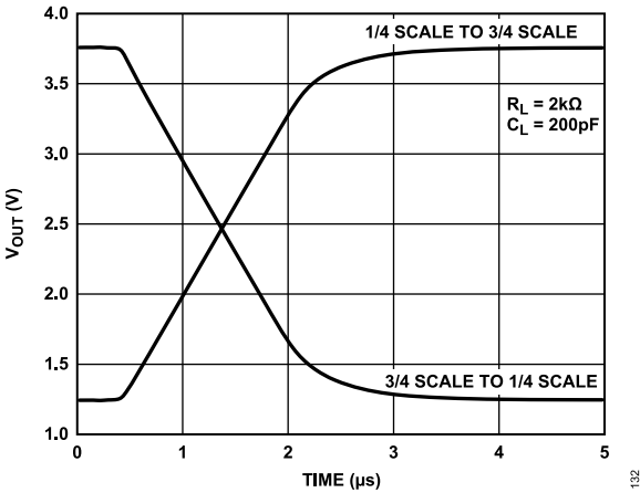
Figure 26. DAC Settling Time, Output Range = 0 V to 2 \times V_{REF}
