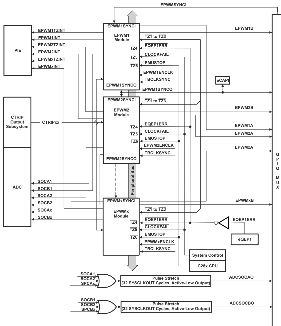
Figure 8-37. ePWM
