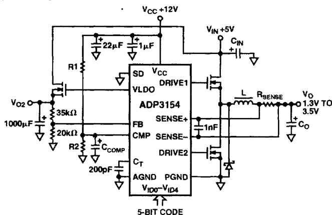
Figure 1. Typical Application
