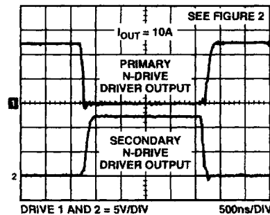
Figure 7. Gate Switching Waveforms
