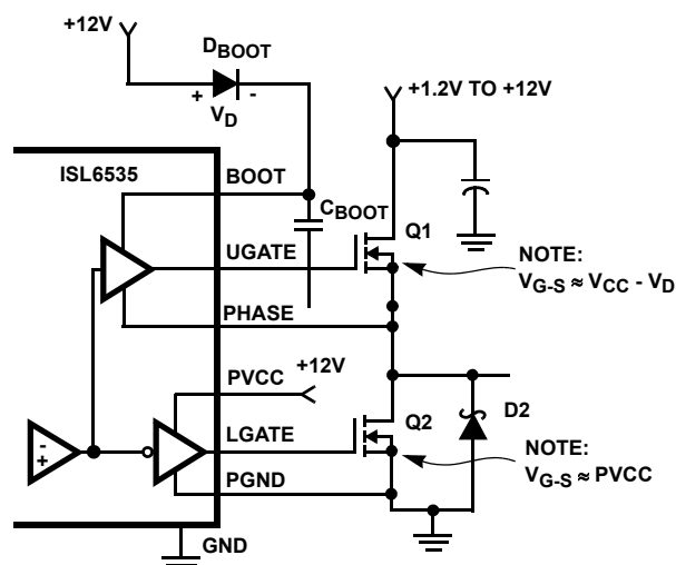
FIGURE 12. UPPER GATE DRIVE - BOOTSTRAP OPTION
