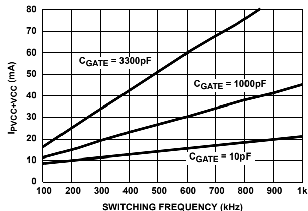
FIGURE 5. BIAS SUPPLY CURRENT vs FREQUENCY
