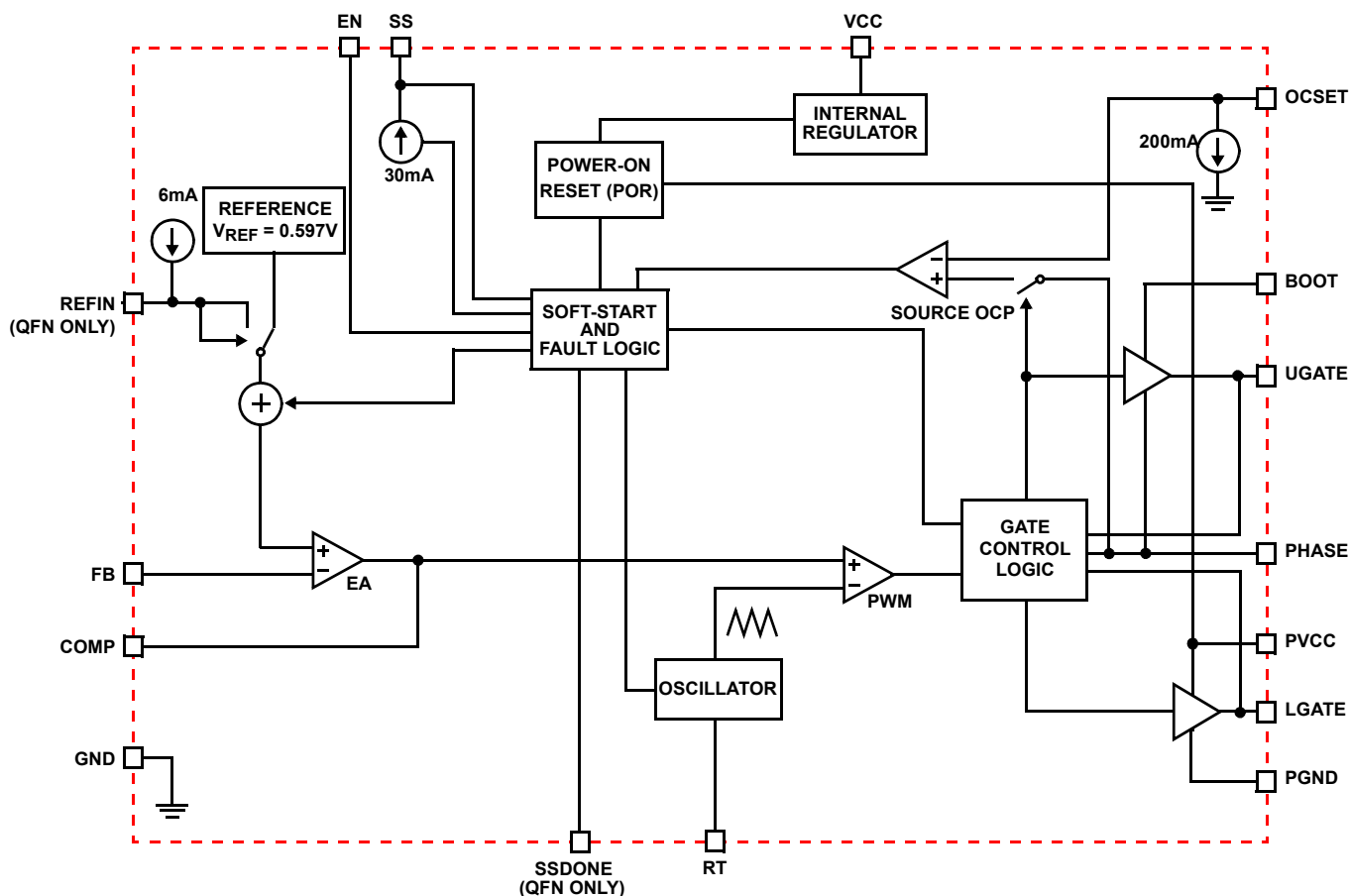
FIGURE 1. BLOCK DIAGRAM
