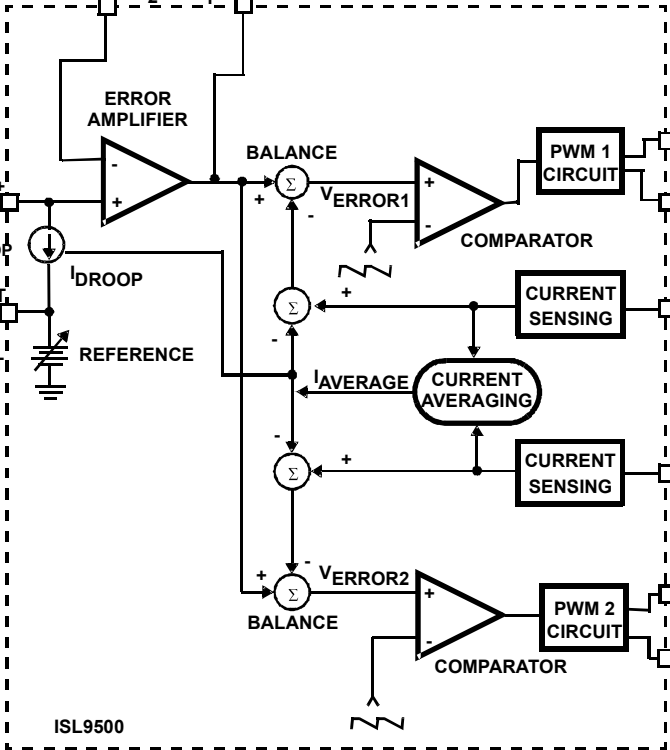
FIGURE 9. SIMPLIFIED BLOCK DIAGRAM OF THE ISL9500 VOLTAGE AND CURRENT CONTROL LOOPS FOR A TWO CHANNEL REGULATOR.
