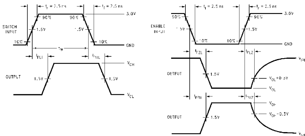
FIGURE 2. AC Waveforms
