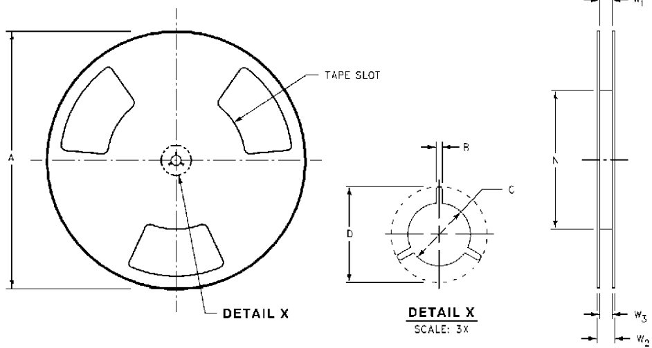
REEL DIMENSIONS inches (millimeters)
