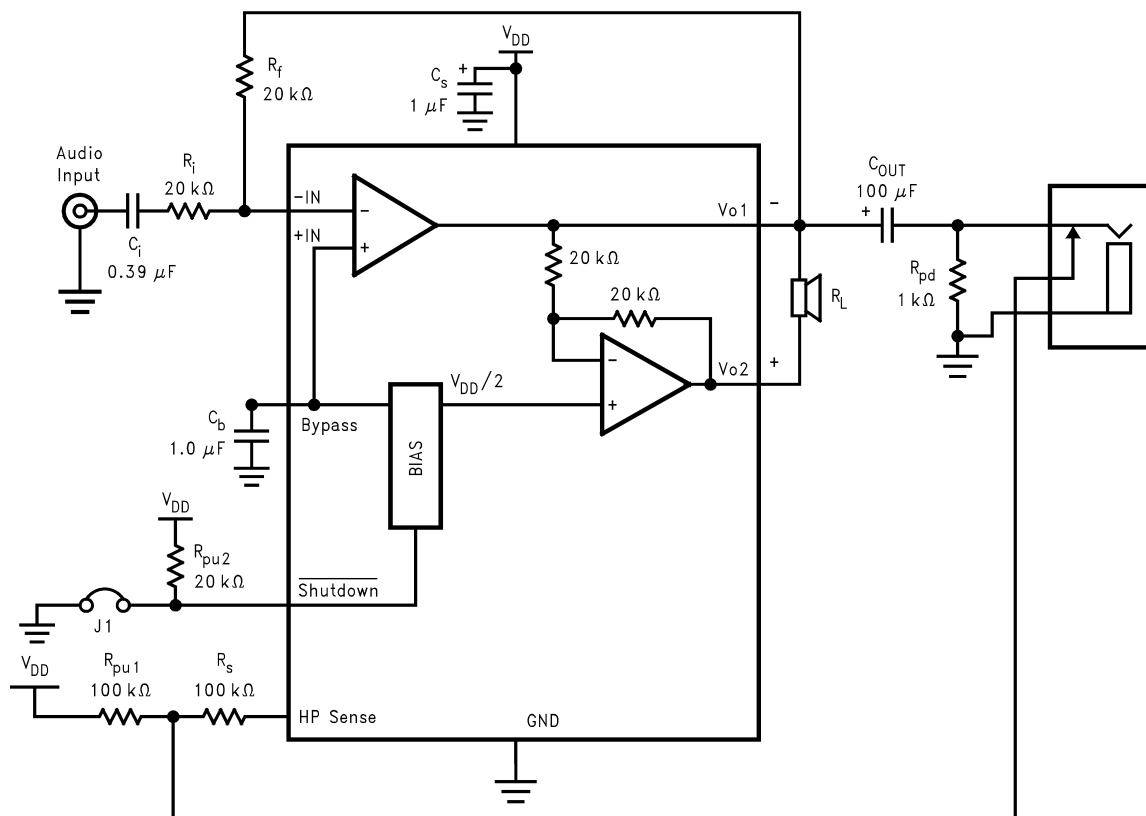
FIGURE 4. Reference Design Schematic For Demo Boards
