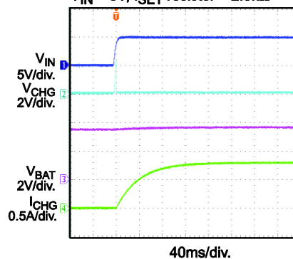
Power Ramps Up vs. Battery Charge
