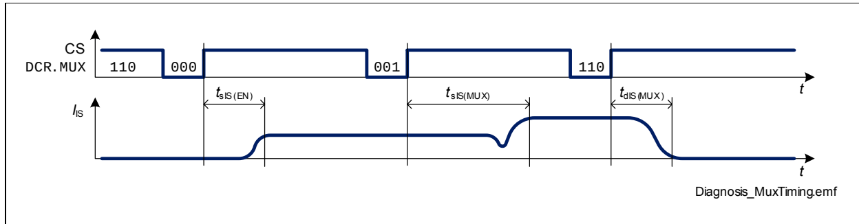
Figure 23 Current Sense Multiplexer Timings
