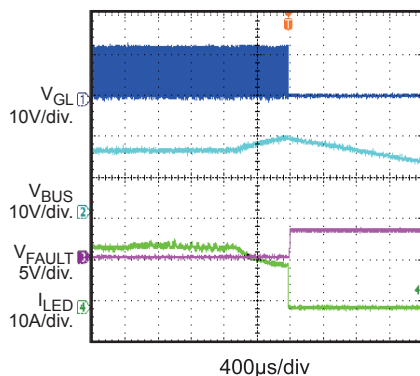
V_{\text{BUS}} OVP Protection
