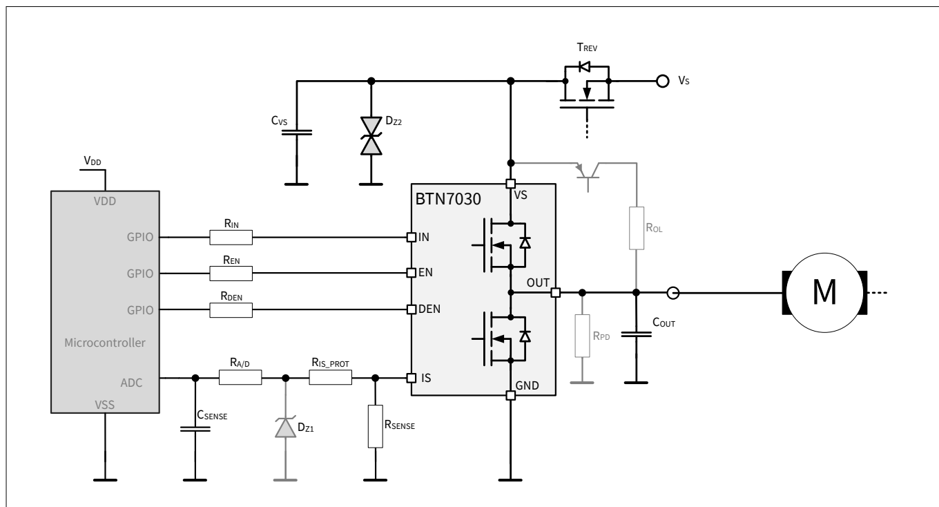
Figure 27 BTN7030-1EPA application diagram
