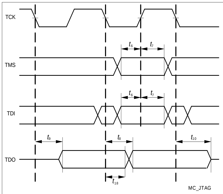
Figure 18 JTAG Timing
