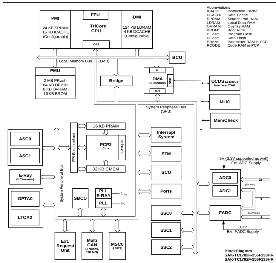
Figure 3 SAK-TC1782F-256F133HR / SAK-TC1782F-256F133HL Block Diagram
