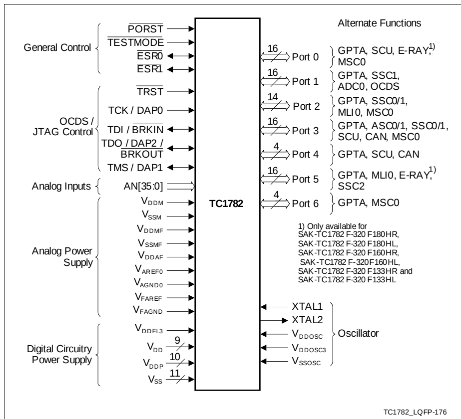
Figure 5 TC1782 Logic Symbol
