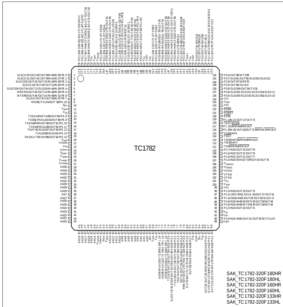
Figure 6 SAK-TC1782F-320F180HR / SAK-TC1782F-320F180HL / SAK-TC1782F-320F160HR / SAK-TC1782F-320F160HL SAK-TC1782F-256F133HR / SAK-TC1782F-256F133HL Pinning
