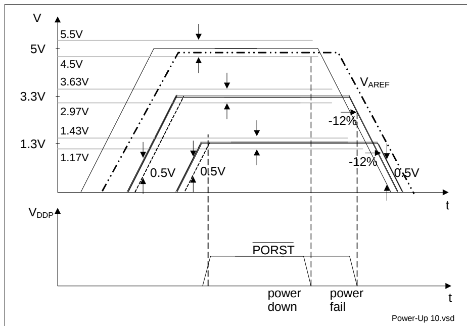
Figure 14 5 V / 3.3 V / 1.3 V Power-Up/Down Sequence for 10% Operating Range
