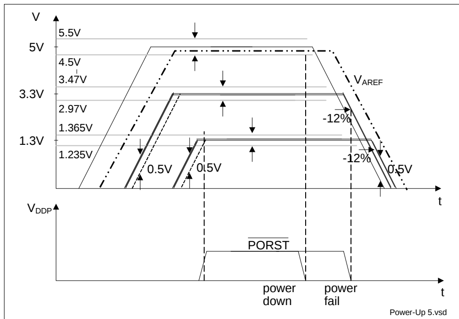
Figure 15 5 V / 3.3 V / 1.3 V Power-Up/Down Sequence for 5% Operating Range
