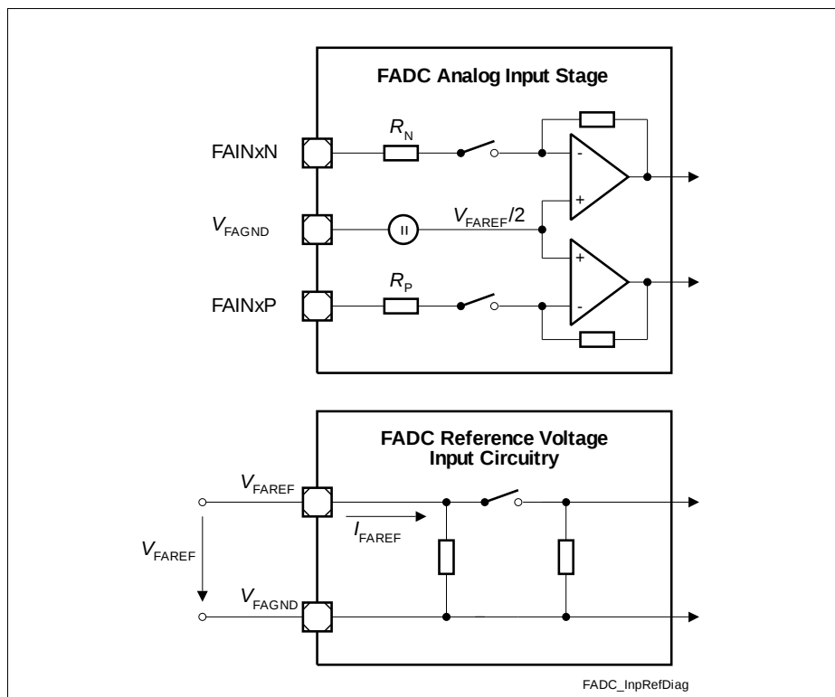
Figure 10 FADC Input Circuits
