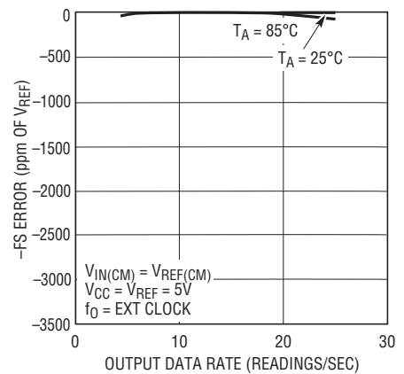
Figure 21. -FS Error vs Output Data Rate and Temperature
