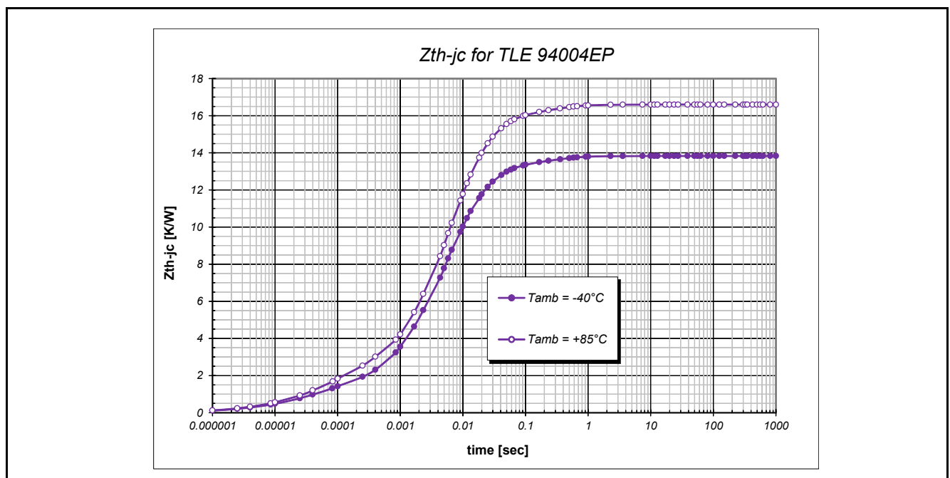
Figure 17 ZthJC Curve
