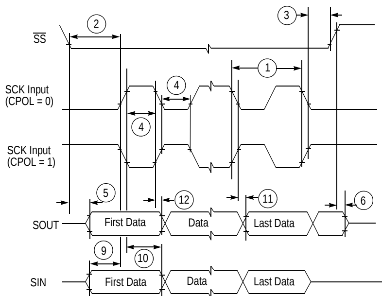
Figure 16. DSPI classic SPI timing — Slave, CPHA = 0
