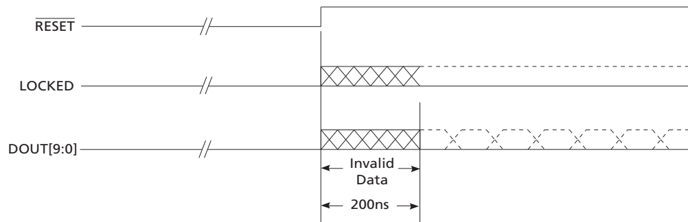
Figure 3-20: Reset Timing
