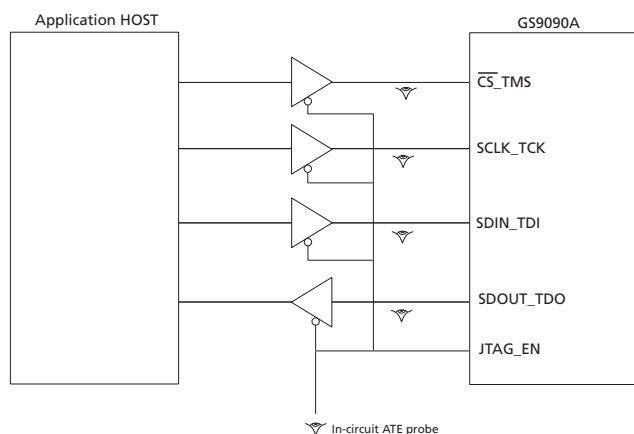
Figure 3-21: In-Circuit JTAG
