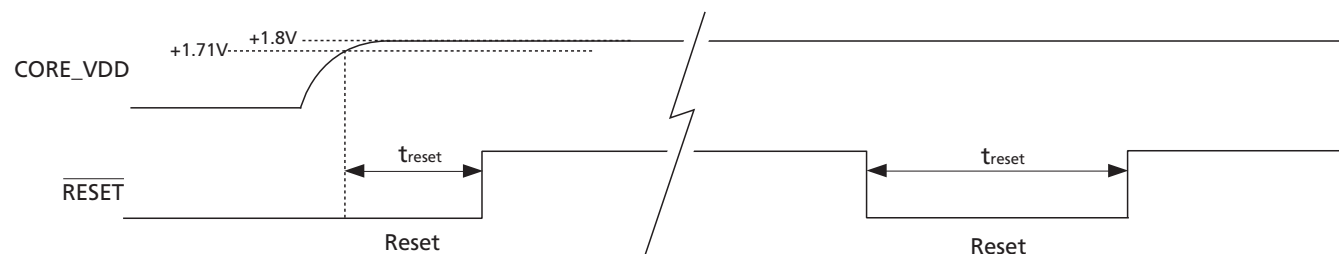
Figure 3-23: Reset pulse
