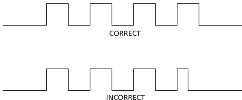
Figure 3-9: Burst Clock
