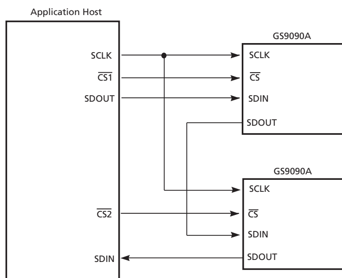
Figure 3-15: GSPI Application Interface Connection
