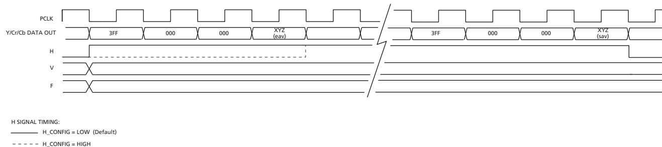
Figure 3-3: H,V,F Timing
