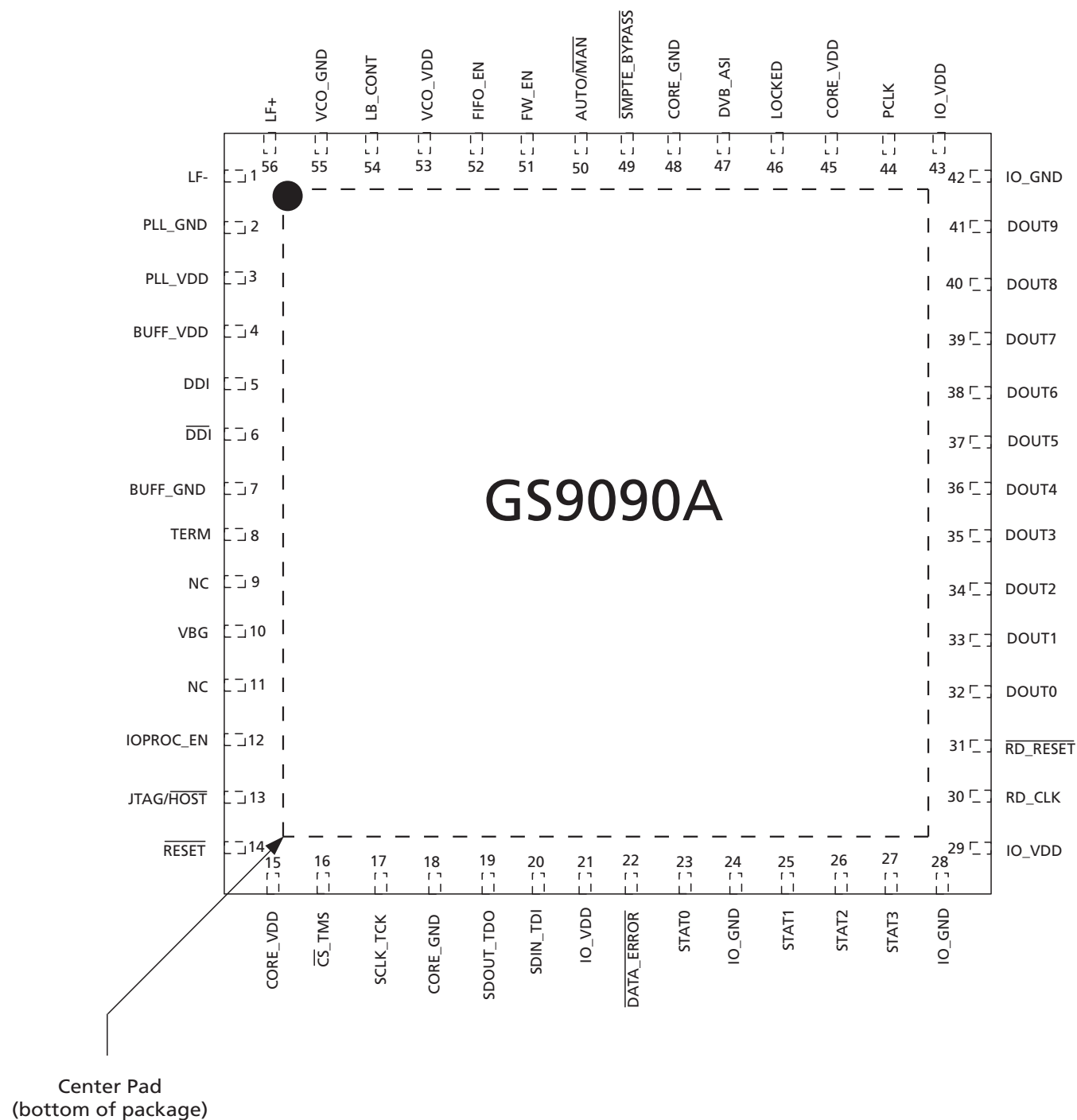
Figure 1-1: Pin Assignment
