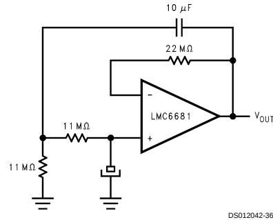
FIGURE 19. LMC6681 Used for Signal Processing
