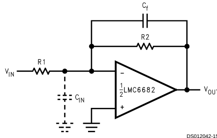
FIGURE 17. Canceling the Effect of Input Capacitance
