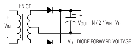
FIGURE 1A. PUSH-PULL RECTIFICATION
