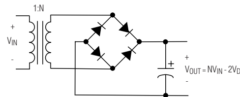
FIGURE 1C. FULL-WAVE RECTIFIER
