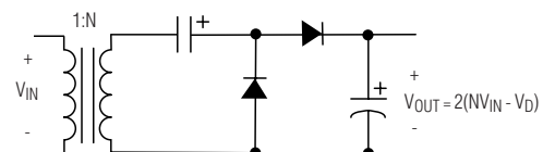
FIGURE 1B. VOLTAGE DOUBLER
