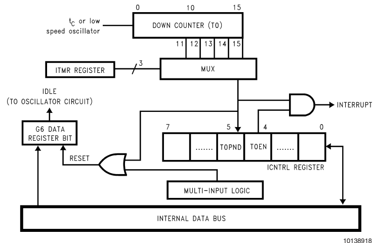
FIGURE 15. Functional Block Diagram for Idle Timer T0
