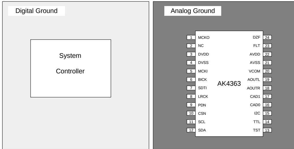
Figure 10. Ground Layout
