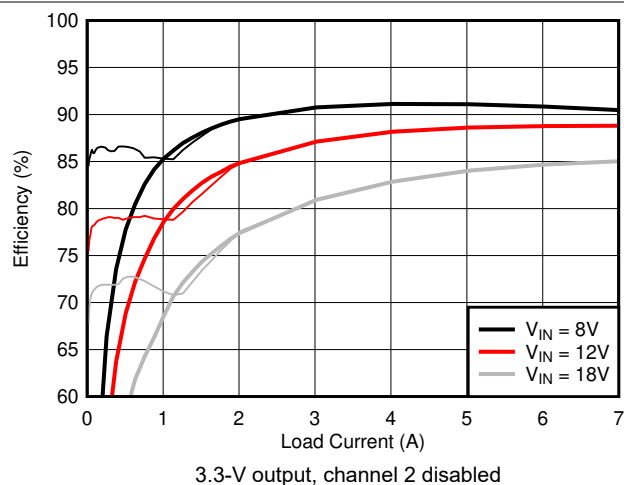
Figure 10-6. Efficiency Versus I_{OUT}
