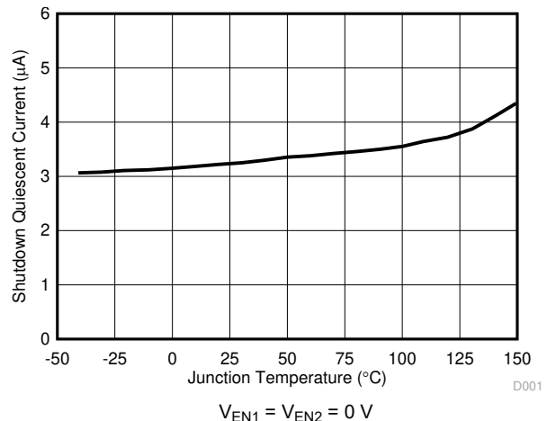
Figure 8-6. Shutdown Current Versus Temperature
