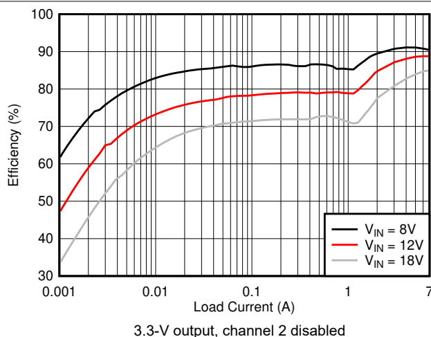
Figure 10-7. Efficiency Versus I_{OUT} , Log Scale
