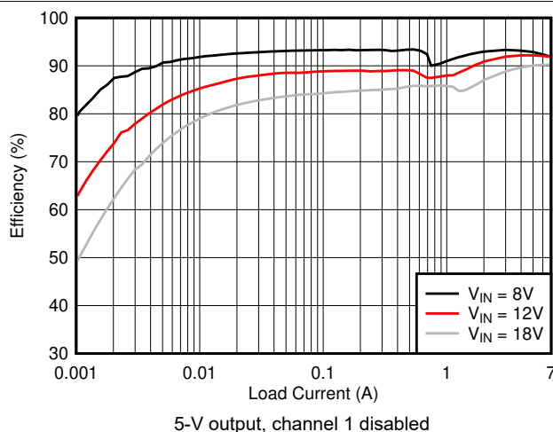
Figure 10-9. Efficiency Versus I_{OUT} , Log Scale
