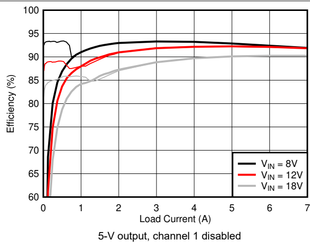
Figure 10-8. Efficiency Versus I_{OUT}
