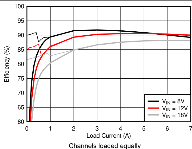
Figure 10-5. Efficiency Versus I_{OUT}
