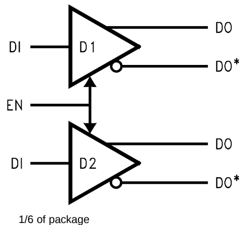
Figure 2. Functional Diagram
