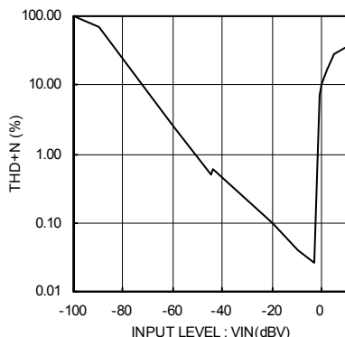
Fig.11 EXTO Total Harmonic Distortion
