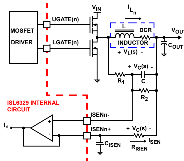
FIGURE 21. DCR SENSING CONFIGURATION
