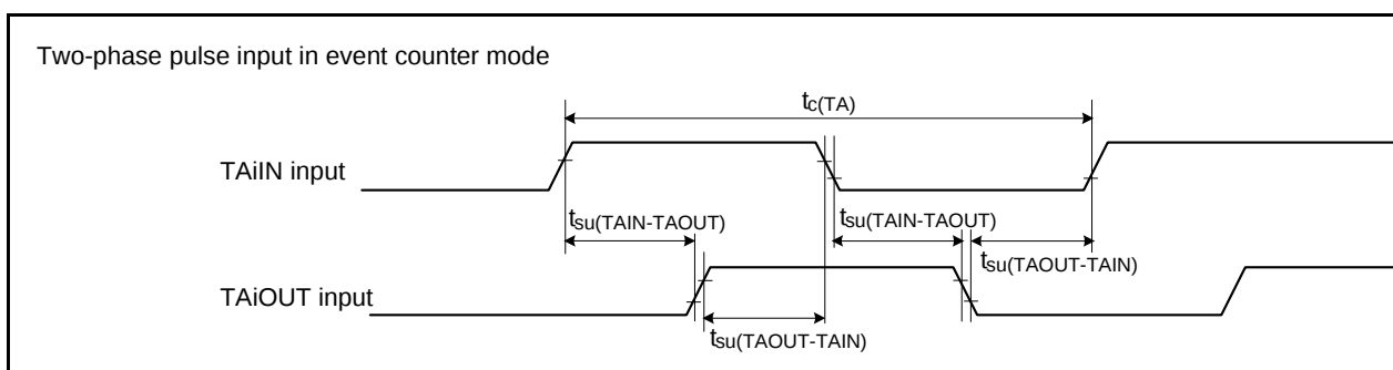
Figure 5.18 Timer A Input (Two-Phase Pulse Input in Event Counter Mode)
