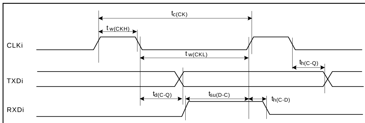
Figure 5.35 Serial Interface
