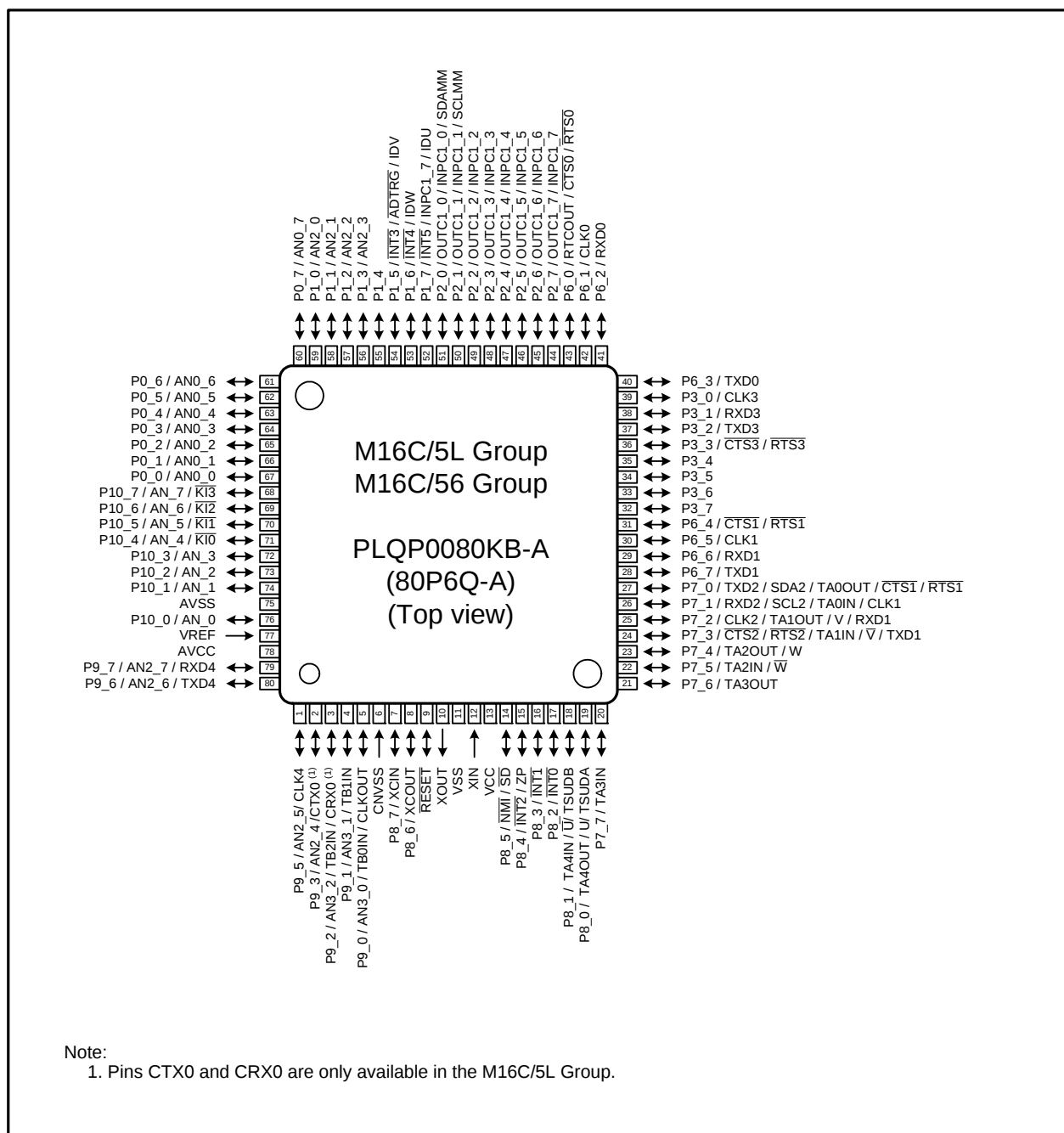
Figure 1.5 Pin Assignment for 80-Pin Package (Top View)
