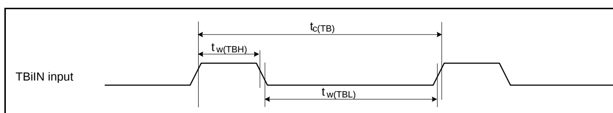
Figure 5.42 Timer B Input
