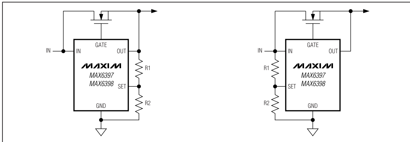
Figure 6. Setting the MAX6397/MAX6398 Overvoltage Threshold
