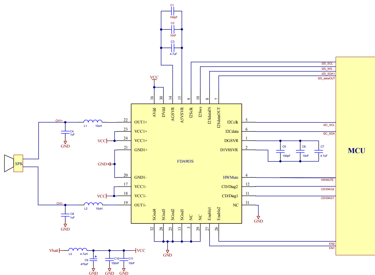
Figure 3. Application diagram
