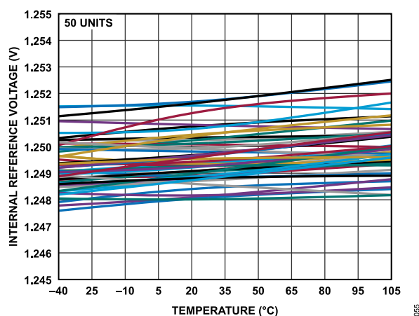
Figure 52. 1.25 V Internal Reference Voltage vs. Temperature
