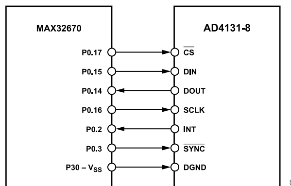
Figure 97. Example of MAX32670 \mu C SPI Connection to AD4131-8
