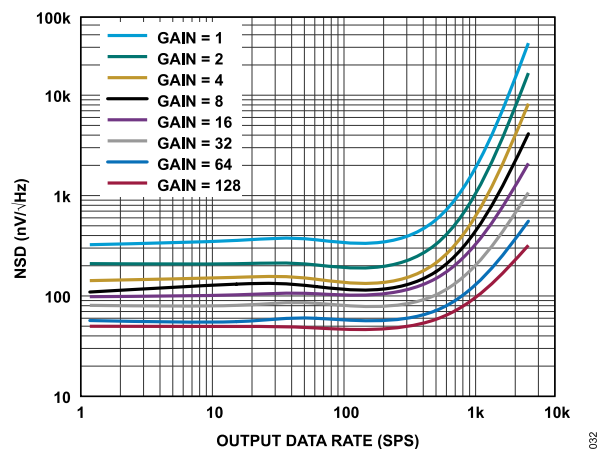
Figure 29. NSD vs. Output Data Rate for Various Gains ( \text{Sinc}^3 Filter, External 2.5 V Reference)
