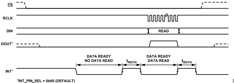
Figure 9. Data Ready High Time when Data Ready is Initially Low and the Next Conversion is Available
