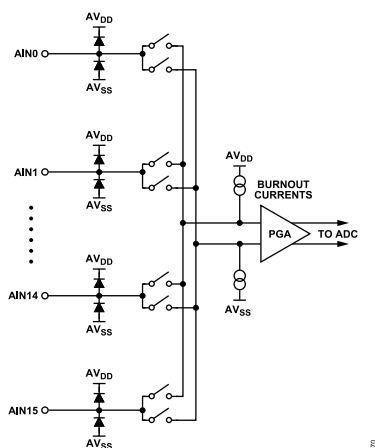
Figure 67. Analog Input Multiplexer Circuit
