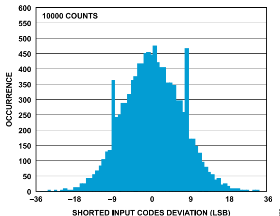
Figure 27. Noise Histogram Plot ( \text{Sinc}^4 Filter, ODR = 240 SPS, Gain = 1, Internal 1.25 V Reference)
