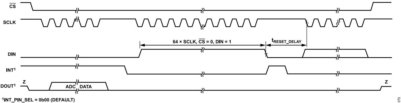
Figure 72. Software Reset Timing Diagram
