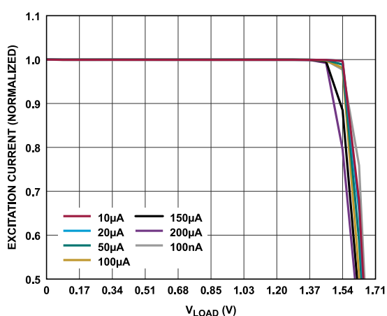
Figure 59. Output Compliance for Various IEXC Sources ( AV_{DD} = 1.71 V, V_{LOAD} is Load Voltage)
