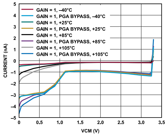
Figure 31. Absolute AINP Current vs. AIN Common-Mode Voltage (VCM) for Various Temperatures (Gain = 1, VDIFF = 0 V)
