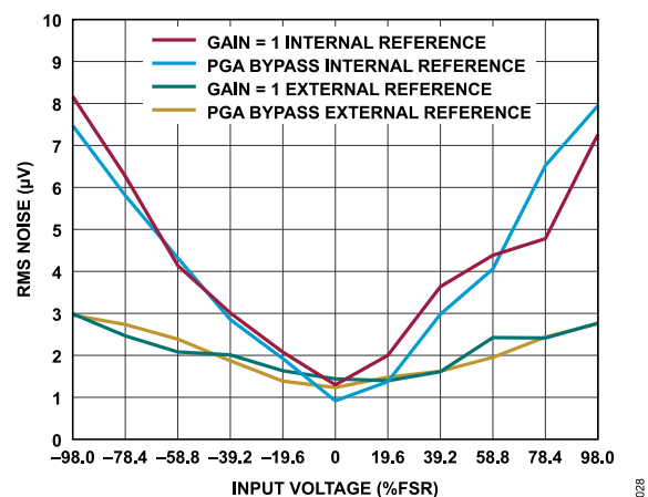
Figure 25. RMS Noise vs. Analog Input Voltage ( \text{Sinc}^3 Filter, ODR = 50 SPS, Gain = 1 and Gain = 1 with PGA Bypass, 2.5 V Reference)
