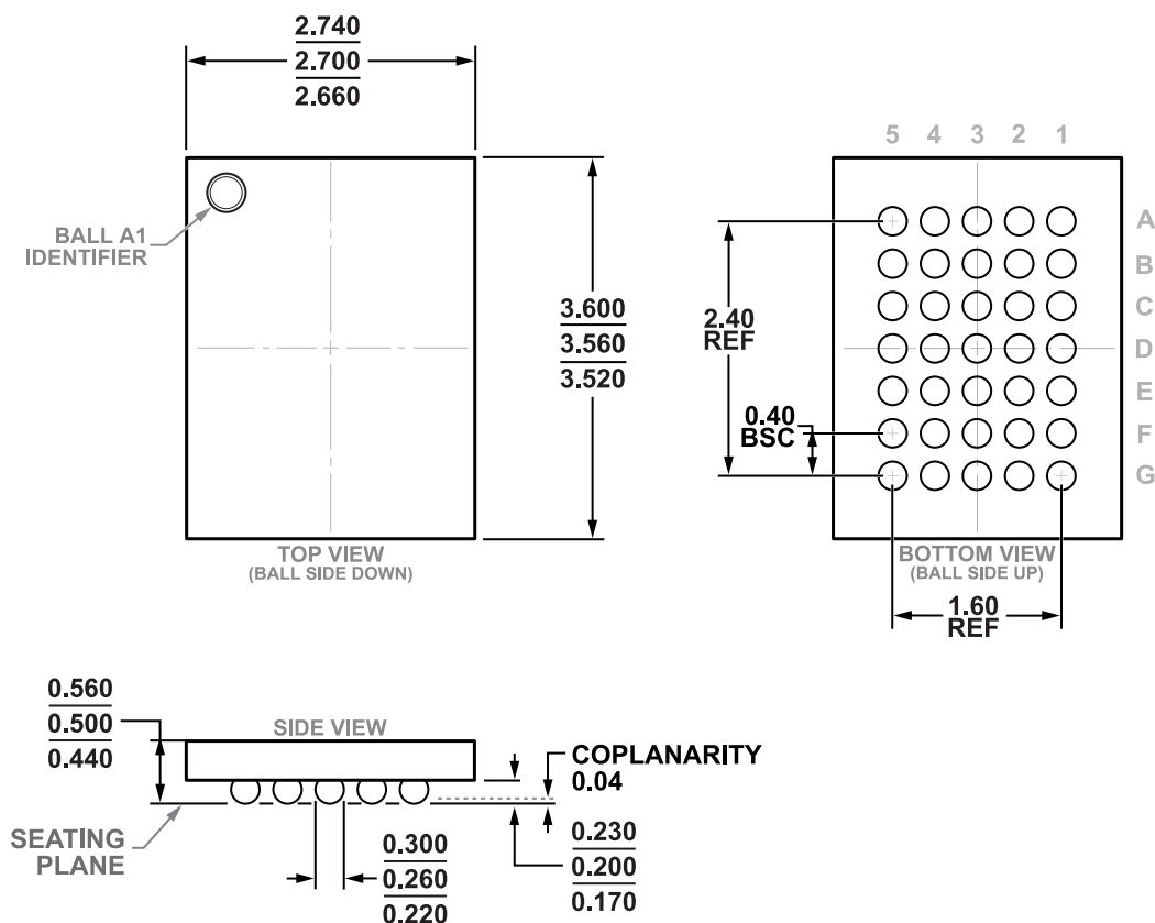
Figure 113. 35-Ball Wafer Level Chip Scale Package [WLCSP] 2.7 mm × 3.56 mm Body and 0.5 mm Package Height (CB-35-3) Dimensions Shown in Millimeters
