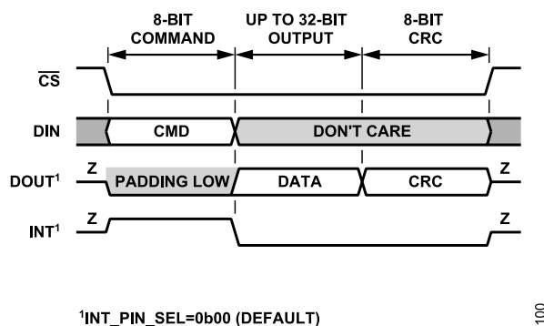
Figure 95. SPI Read Transaction with CRC
