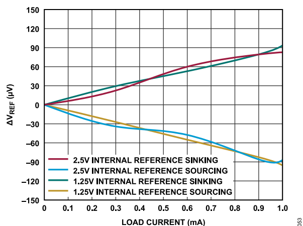
Figure 50. 1.25 V ( AV_{DD} = 1.8 V) and 2.5 V ( AV_{DD} = 3.3 V) Internal Reference Voltage vs. Load Current
