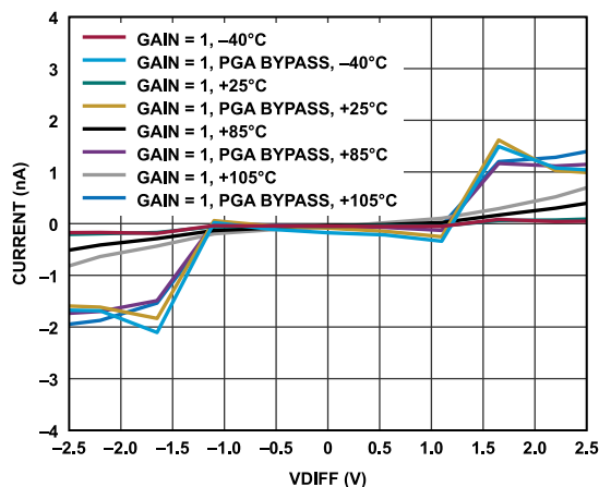
Figure 32. Differential AIN Current vs. VDIFF for Various Temperatures (Gain = 1, VCM = AV_{DD}/2 )
