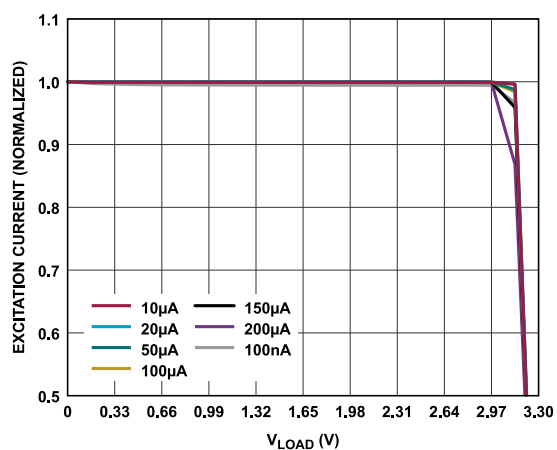
Figure 56. Output Compliance for Various IEXC Sources ( AV_{DD} = 3.3 V, V_{LOAD} is Load Voltage)
