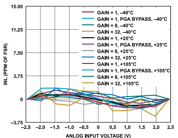
Figure 22. INL Error vs. Differential Input Amplitude for Various Gains and Temperatures (Sinc 3 Filter, ODR = 50 SPS, External 2.5 V Reference)
