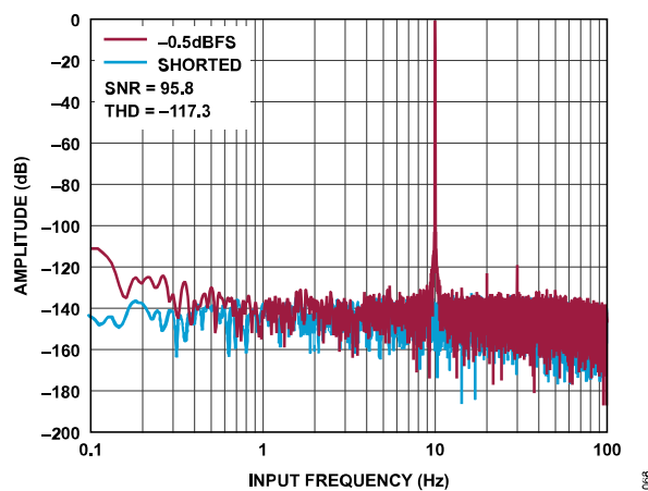
Figure 65. FFT, -0.5 dBFS vs. Shorted Inputs, 10 Hz Input Tone, \text{Sinc}^3 Filter, ODR = 240 SPS, Gain = 1, External Reference
