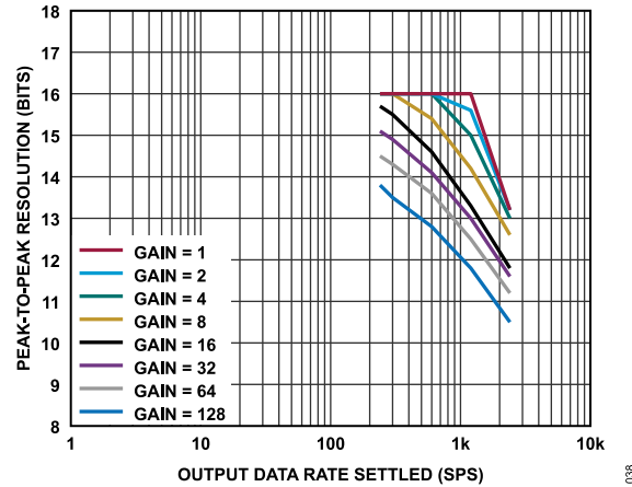
Figure 62. Peak-to-Peak Resolution vs. Output Data Rate (Settled) for Various Gains (Sinc 4 Filter)
