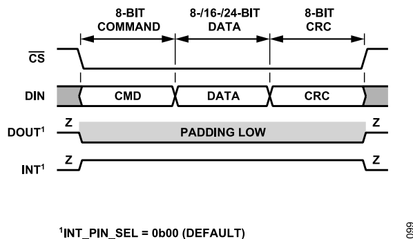
Figure 94. SPI Write Transaction with CRC
