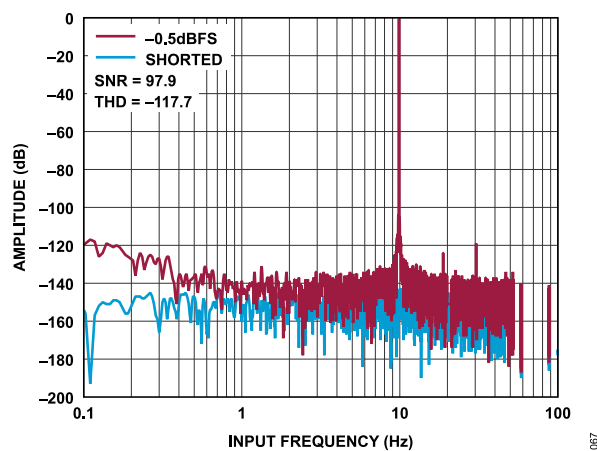
Figure 64. FFT, -0.5 dBFS vs. Shorted Inputs, 10 Hz Input Tone, \text{Sinc}^3 Filter, ODR = 240 SPS, Gain = 1, Internal Reference
