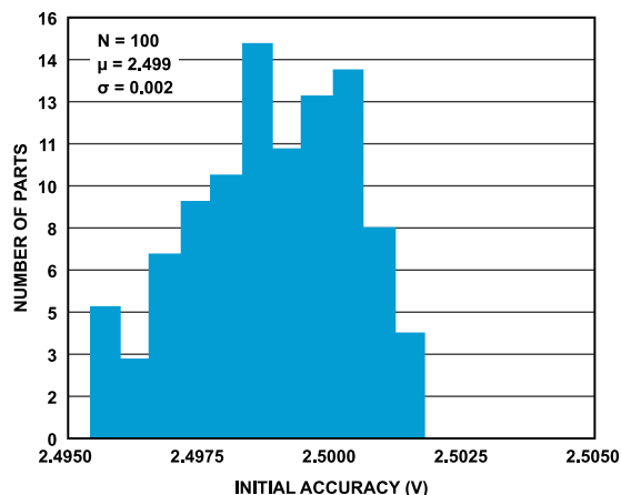
Figure 48. 2.5 V Internal Reference Voltage Histogram
