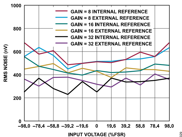
Figure 26. RMS Noise vs. Analog Input Voltage ( \text{Sinc}^3 Filter, ODR = 50 SPS, Gain = 8, Gain = 16 and Gain = 32, 1.25 V Reference)
