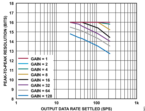
Figure 63. Peak-to-Peak Resolution vs. Output Data Rate (Settled) for Various Gains (Sinc 4 + Sinc 1 Filter)
