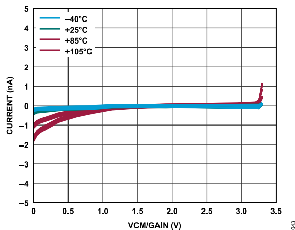
Figure 40. Absolute AINM Current vs. VCM/Gain for Various Temperatures (Gain = 2 to 128, VDIFF = 0 V)
