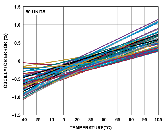
Figure 23. Internal Oscillator Error vs. Temperature
