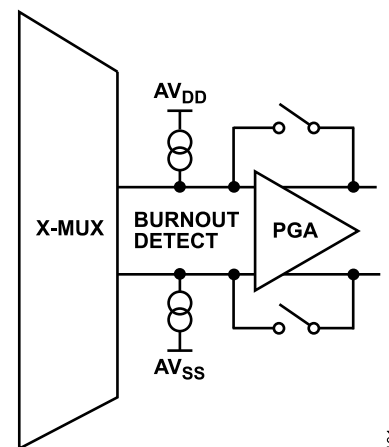
Figure 96. Burnout Currents
