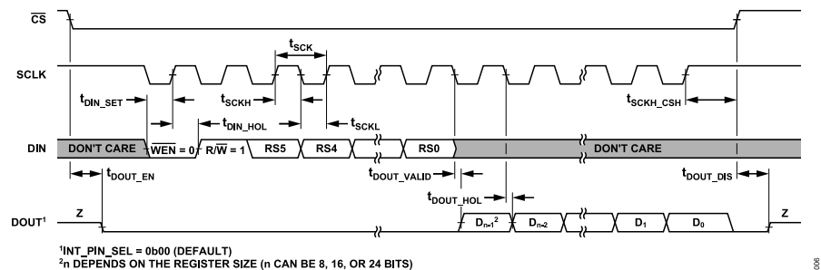
Figure 6. 3-Wire Mode Read Cycle Timing Diagram, 3-Wire Mode (CSB_EN Bit Set to 0), CS Pin Used to Tristate the DOUT Pin
