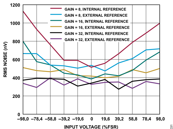
Figure 28. RMS Noise vs. Analog Input Voltage ( \text{Sinc}^3 Filter, ODR = 50 SPS, Gain = 8, Gain = 16 and Gain = 32, 2.5 V Reference)
