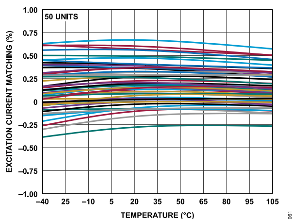
Figure 58. Excitation Current Matching vs. Temperature (100 \mu A)
