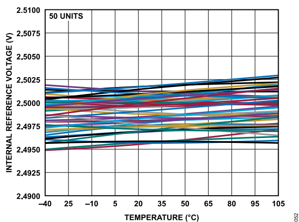
Figure 49. 2.5 V Internal Reference Voltage vs. Temperature
